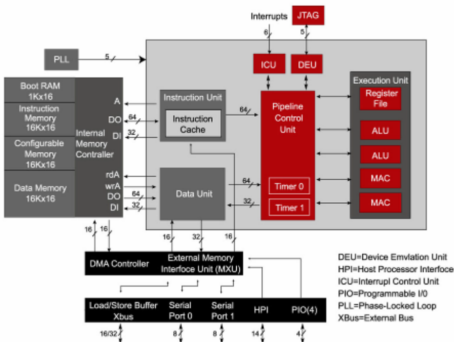
Figure 1. VSI403US Functional Block Diagram
